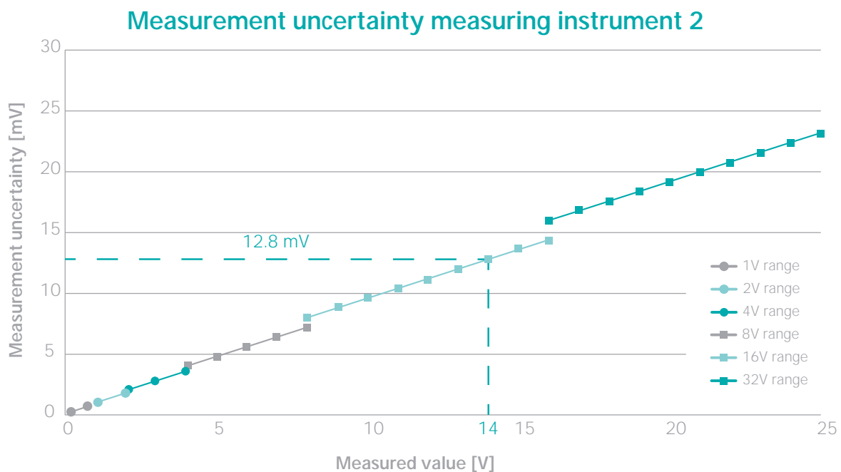
Figure 4: Measuring instrument 2 has a larger number of measuring ranges.
