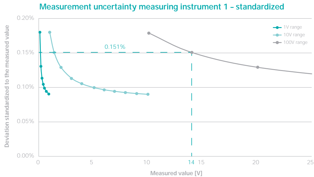
Figure 5: Standardized representation of the measurement uncertainty for measuring instrument 1.
