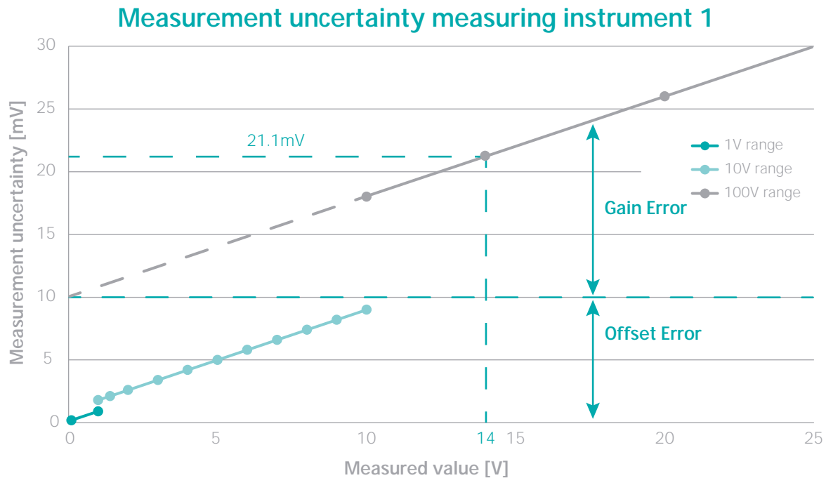
Figure 3: The absolute error measured on measuring instrument 1.
