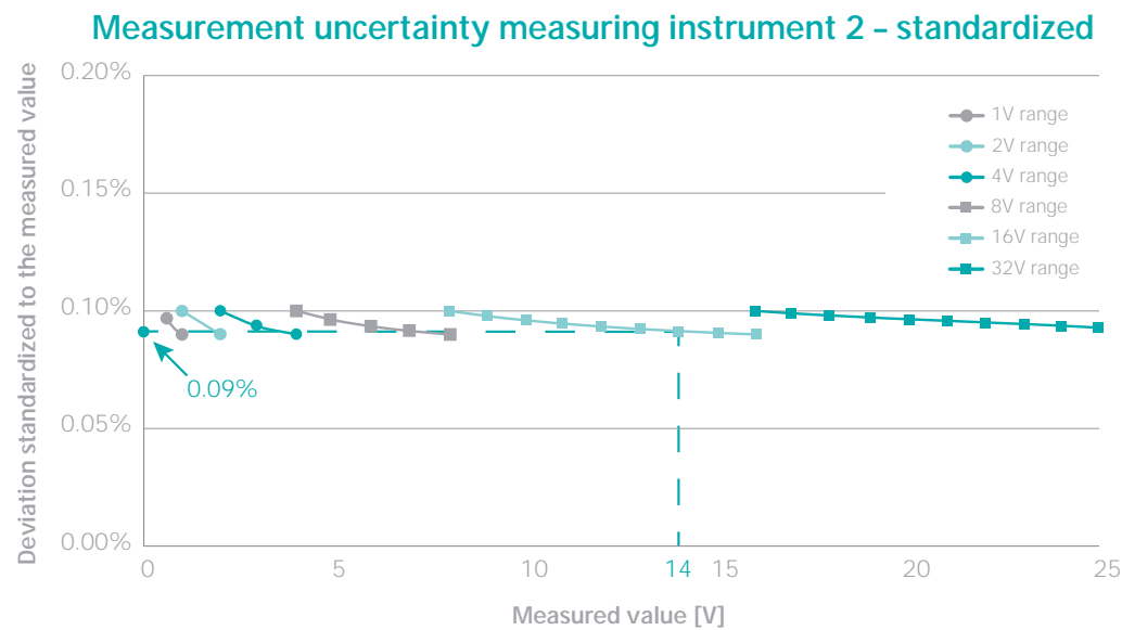
Figure 6: Standardized representation of the measurement uncertainty for measuring instrument 2.
